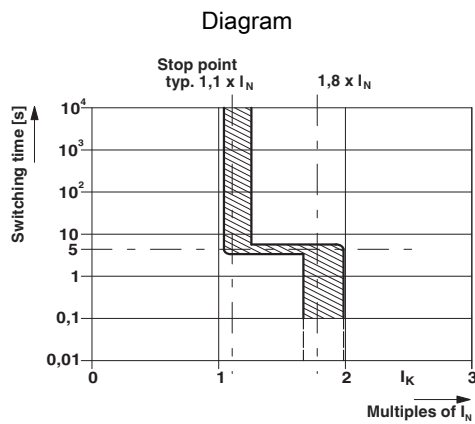
Trigger characteristic
