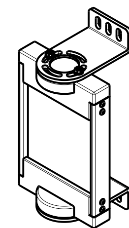
ISOMETRIC VIEW SCALE 1:4
